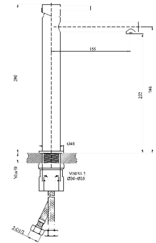
HM 2809 MB Single-lever Basin Faucet H & C Rp. 1.500.000
