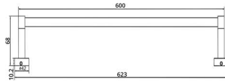
Single Towel Bar • Material : Brass • Polished : Chrome & Matte Black
