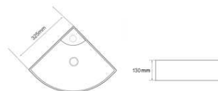
Wall-hung Wash Basin • Ceramic Material • Smooth Surface • Size : 325x130mm
