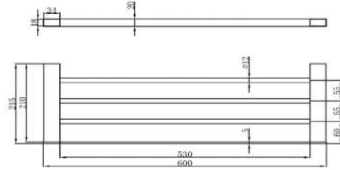
Towel Rack • Material : Brass • Polished : Chrome
