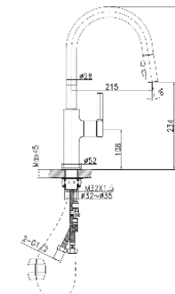
Pull-out Single-lever Kitchen H & C • Material : Brass • Valve Type : Cartridge • Polished : Matte Black
