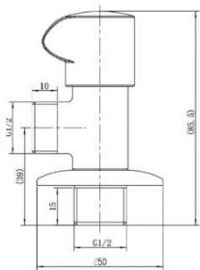
HM 128 Angle Valve • Material : Brass • Usage : Long-term use • Polished : Chrome Rp. 149.000
