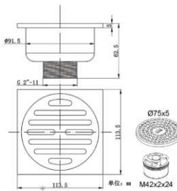
HMS 01 BK Floor Drainer • Material : Brass • Usage : Long-term use • Polished : Black Rp. 700.000
