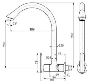
In-wall Kitchen Faucet ( Cold ) • Material : Brass • Valve Type : Cartridge • Polished : Chrome
