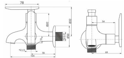
Two Function Faucet Cold • Material : Brass • Valve Type : Cartridge • Polished : Chrome
