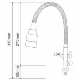
Single-lever Kitchen Cold Tap • Material : Brass • Valve Type : Cartridge • Polished : Chrome
