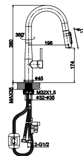
HM 1100 MW Pull-out Single-lever Kitchen H & C Rp.
