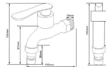
Washer Bibcock • Material : Brass • Valve Type : Cartridge • Polished : Chrome
