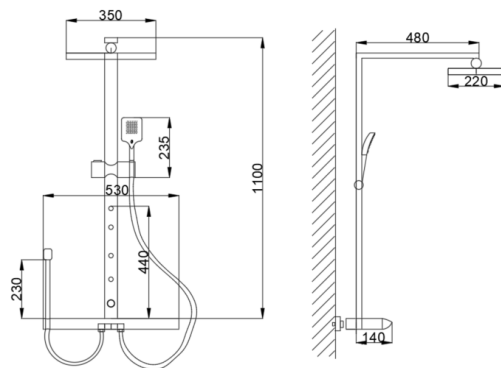
HM 0119 Shower Column Set Thermostatic ( H & C ) Rp. 12.500.000
