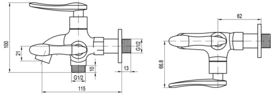
Two Function Faucet Cold • Material : Brass • Valve Type : Cartridge • Polished : Black
