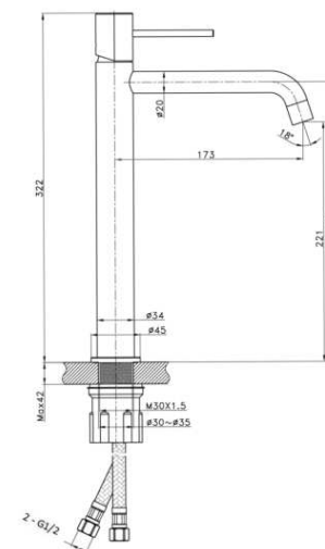
HM 1527 MB Single-lever Basin Faucet H & C Rp. 2.200.000
