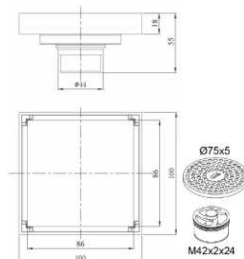
HMS 10 GM Floor Drainer • Material : Brass • Usage : Long-term use • Polished : Grey Matte Rp. 616.000
