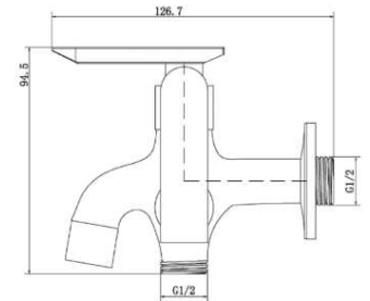
Two Function Faucet Cold • Material : Brass • Valve Type : Cartridge • Polished : Chrome
