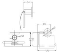
Roll Holder • Material : Stainless Steel SUS 304 • Polished : Chrome
