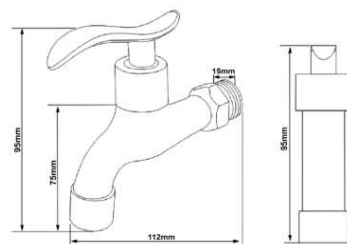
Washer Bibcock • Material : Brass • Valve Type : Cartridge • Polished : Chrome
