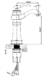
HM 1481 G Single-lever Basin Faucet H & C • Material : Brass • Valve Type : Cartridge • Polished : Gold Rp. 2.700.000
