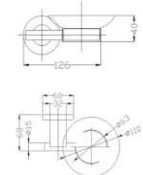
Soap Dish Holder • Material : Stainless Steel SUS 304 • Polished : Chrome
