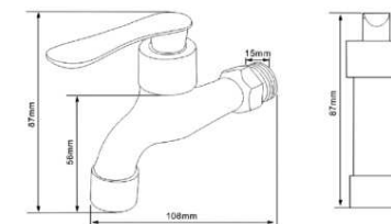
Washer Bibcock • Material : Brass • Valve Type : Cartridge • Polished : Chrome
