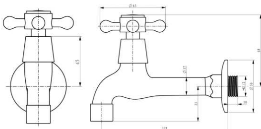
Washer Bibcock • Material : Brass • Valve Type : Cartridge • Polished : Chrome
