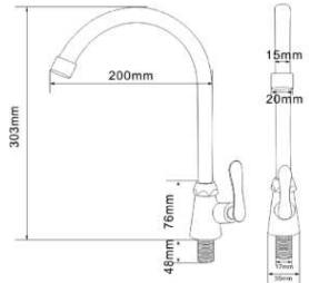
Single-lever Kitchen Cold Tap • Material : Brass • Valve Type : Cartridge • Polished : Chrome
