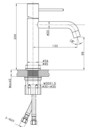
HM 1526 MB Single-lever Basin Faucet H & C Rp. 1.650.000
