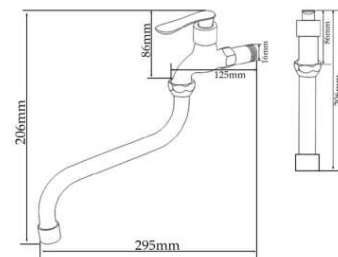
In-wall Kitchen Faucet ( Cold ) • Material : Brass • Valve Type : Cartridge • Polished : Chrome
