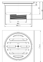
HMS 01 BK Floor Drainer • Material : Brass • Usage : Long-term use • Polished : Black Rp. 700.000
