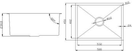
WGHMS 5845 Topmount & Undermount - Single Large Bowl Sink Start From Rp. 1.500.000
