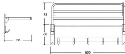
Towel Bar • Material : Brass • Polished : Chrome & Matte Black
