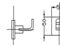
Single Robe Hook • Material : Stainless Steel SUS 304 • Polished : Chrome
