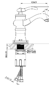
HM 1482 G Single-lever Basin Faucet H & C • Material : Brass • Valve Type : Cartridge • Polished : Gold Rp. 2.400.000
