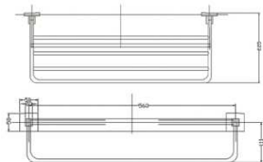
Towel Rack • Material : Stainless Steel SUS 304 • Polished : Chrome
