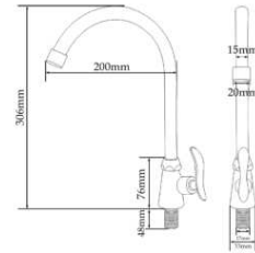
Single-lever Kitchen Cold Tap • Material : Brass • Valve Type : Cartridge • Polished : Chrome
