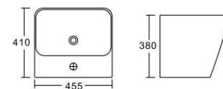
Wall-hung Wash Basin • Ceramic Material • Smooth Surface • Size : 380x410x455mm
