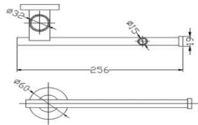
Towel Rack • Material : Stainless Steel SUS 304 • Polished : Chrome
