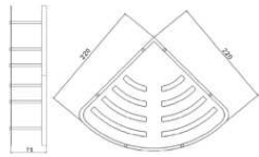
Soap Basket • Material : Stainless Steel SUS 304 • Polished : Chrome & Matte Black
