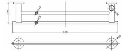
Double Towel Bar • Material : Stainless Steel SUS 304 • Polished : Chrome
