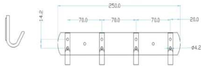
Hook Clothes • Material : Stainless Steel SUS 304 • Polished : Chrome & Matte Black
