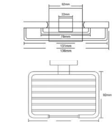
Soap Basket • Material : Stainless Steel SUS 304 • Polished : Chrome & Matte Black
