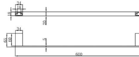
Single Towel Bar • Material : Brass • Polished : Chrome
