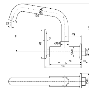
In-wall Kitchen Faucet ( Cold ) • Material : Brass • Valve Type : Cartridge • Polished : Chrome
