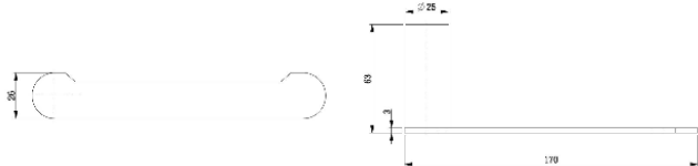
HMYS 3421 CH Roll Holder Rp. 430.000 HMYS 3421 BG Roll Holder Rp. 500.000 HMYS 3421 GM Roll Holder Rp. 480.000 Roll Holder • Material : Brass • Polished : Chrome, Brush Gold, & Gun Metal
