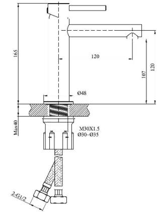
HM 2808 MB Single-lever Basin Faucet H & C Rp. 1.200.000
