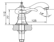
HM 1483 G Triple-hole Basin Faucet H & C • Material : Brass • Valve Type : Cartridge • Polished : Gold Rp. 4.300.000
