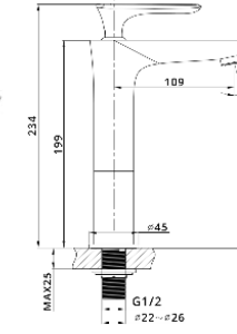
Single-lever Basin Cold Tap • Material : Brass • Valve Type : Cartridge • Polished : Chrome
