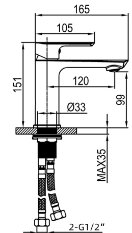
HM 1101 GM Single-lever Basin Faucet H & C Rp. 2.200.000
