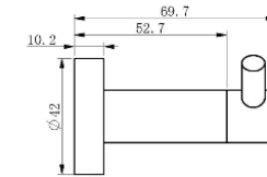
Double Robe Hook • Material : Brass • Polished : Chrome & Black
