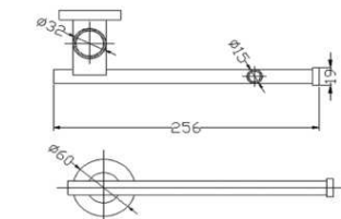
Towel Rack • Material : Brass • Polished : Chrome
