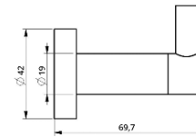
Single Robe Hook • Material : Brass • Polished : Chrome & Black
