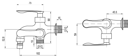
Two Function Faucet Cold • Material : Brass • Valve Type : Cartridge • Polished : Black
