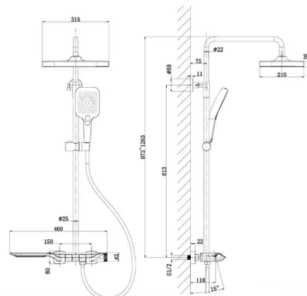
HM 0118 Shower Column Set Thermostatic ( H & C ) Rp. 8.200.000
