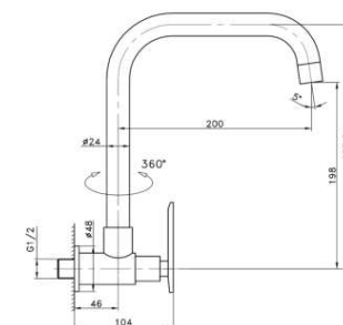
In-wall Kitchen Faucet Flexible ( Cold ) • Material : Brass • Valve Type : Cartridge • Polished : Chrome
