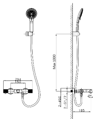
HM 1975 G Single-lever Bath Mixer H&C Rp. 5.500.000
