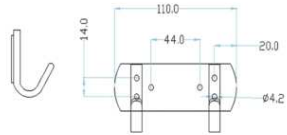
Hook Clothes • Material : Stainless Steel SUS 304 • Polished : Chrome & Matte Black
