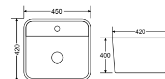
Wall-hung Wash Basin • Ceramic Material • Smooth Surface • Size : 400x420x450mm
