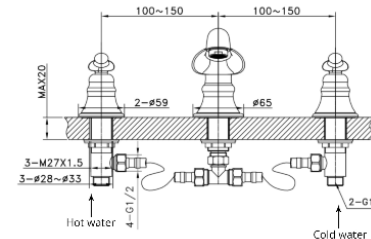
HM 1483 CH Triple-hole Basin Faucet H & C • Material : Brass • Valve Type : Cartridge • Polished : Chrome Rp. 3.800.000
