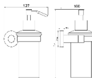
Soap Dispenser • Material : Stainless Steel SUS 304 • Polished : Chrome
