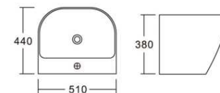
Wall-hung Wash Basin • Ceramic Material • Smooth Surface • Size : 380x440x510mm
