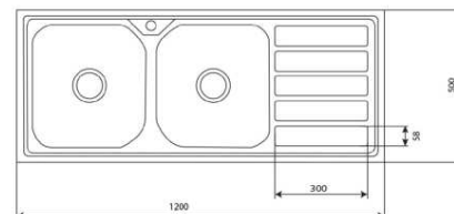
WGS 12050 Topmount - Double Bowl Sink Start From Rp. 1.200.000
