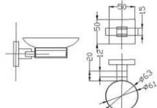
Soap Dish Holder • Material : Stainless Steel SUS 304 • Polished : Chrome
