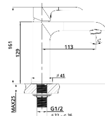
Single-lever Basin Cold Tap • Material : Brass • Valve Type : Cartridge • Polished : Chrome
