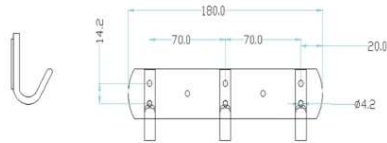
Hook Clothes • Material : Stainless Steel SUS 304 • Polished : Chrome & Matte Black
