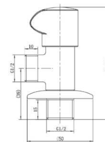
HMF 123 Angle Valve • Material : Brass • Usage : Long-term use • Polished : Chrome Rp. 298.000
