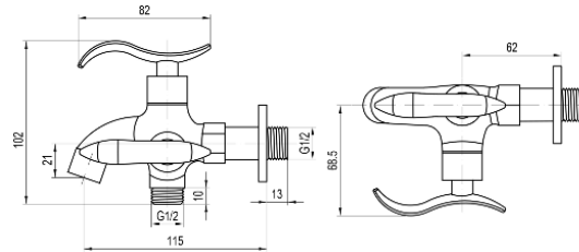
Two Function Faucet Cold • Material : Brass • Valve Type : Cartridge • Polished : Black
