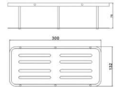
Soap Basket • Material : Stainless Steel SUS 304 • Polished : Chrome & Matte Black
