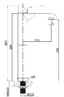
Single-lever Basin Cold Tap • Material : Brass • Valve Type : Cartridge • Polished : Chrome
