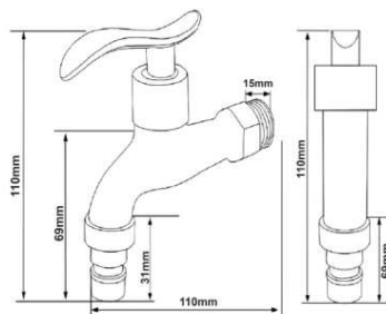
Washer Bibcock • Material : Brass • Valve Type : Cartridge • Polished : Chrome
