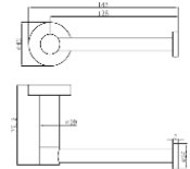
Towel Rack Paper • Material : Stainless Steel SUS 304 • Polished : Chrome
