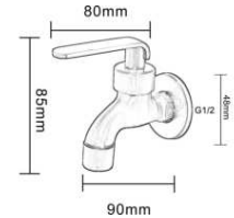
Bibcock Faucet Cold • Material : Brass • Valve Type : Cartridge • Polished : Black
