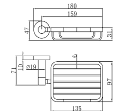
Soap Basket • Material : Stainless Steel SUS 304 • Polished : Chrome & Matte Black
