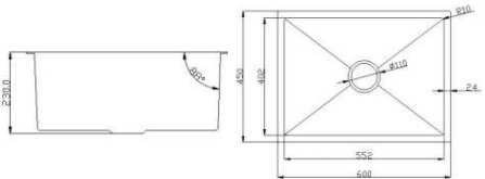
WGHMS 6045 Topmount & Undermount - Single Large Bowl Sink Start From Rp. 1.800.000
