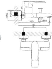
HM 295 Single-lever Bath Mixer H&C ( body only ) Rp. 2.310.000
