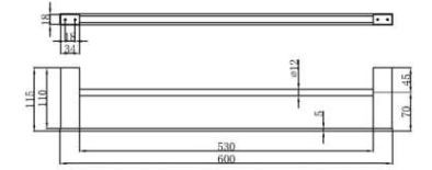
Double Towel Bar • Material : Brass • Polished : Chrome
