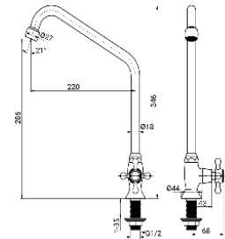
Single-lever Kitchen Cold Tap • Material : Brass • Valve Type : Cartridge • Polished : Chrome
