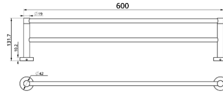
Double Towel Bar • Material : Brass • Polished : Chrome & Matte Black
